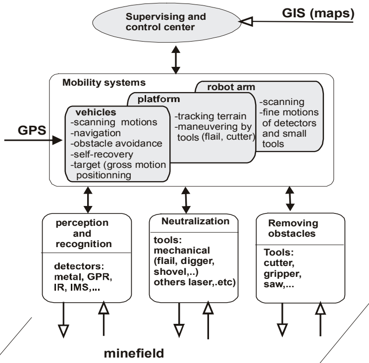
Fig. 2 Parts of the robotic demining system
