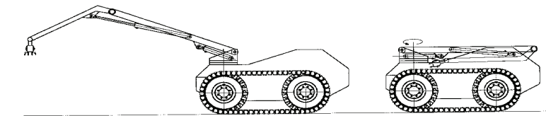
c) The long reach robot arm
